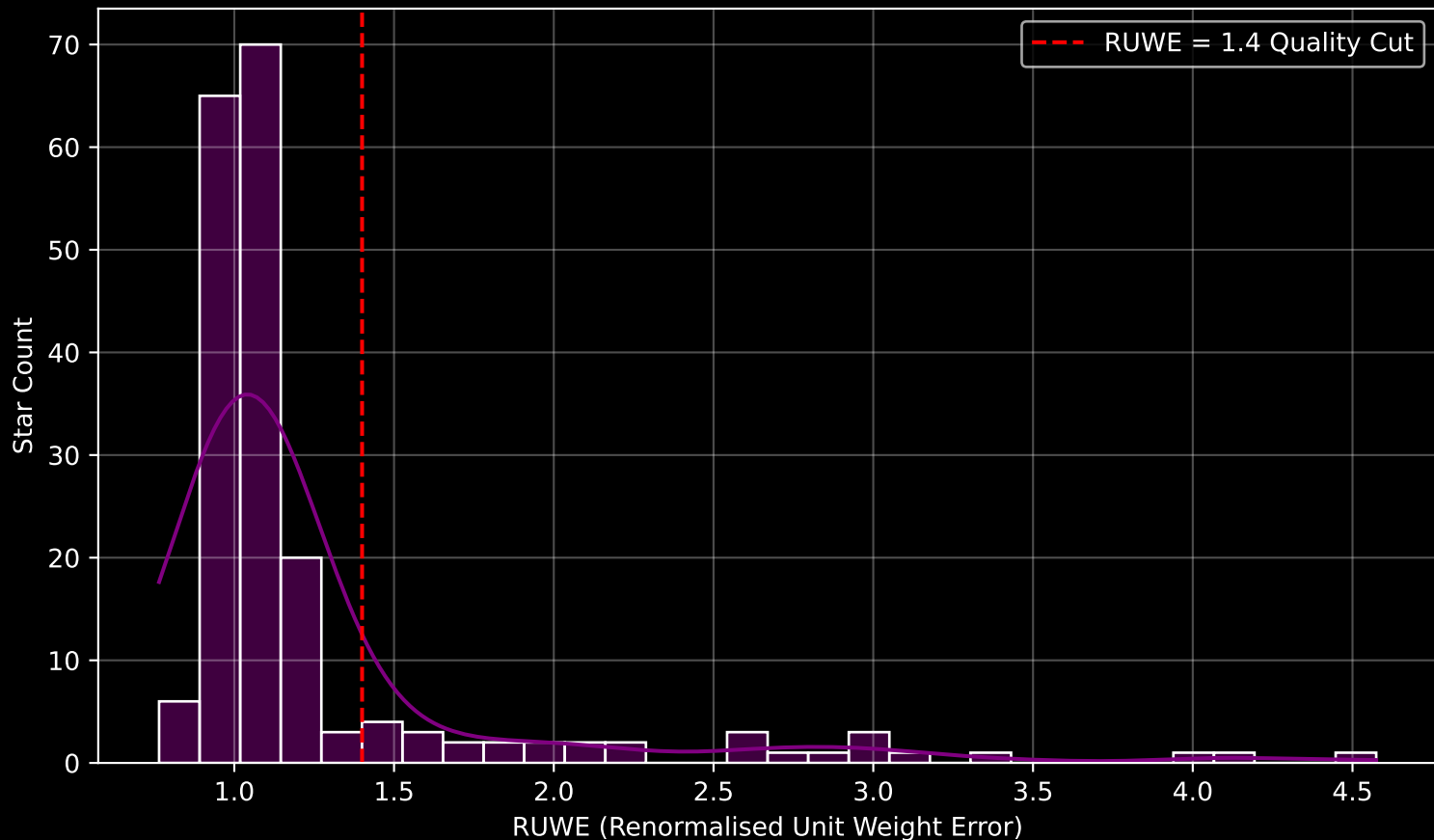
GAPOGEE DR17 Field [260+55] RUWE Distribution (n= 194)
