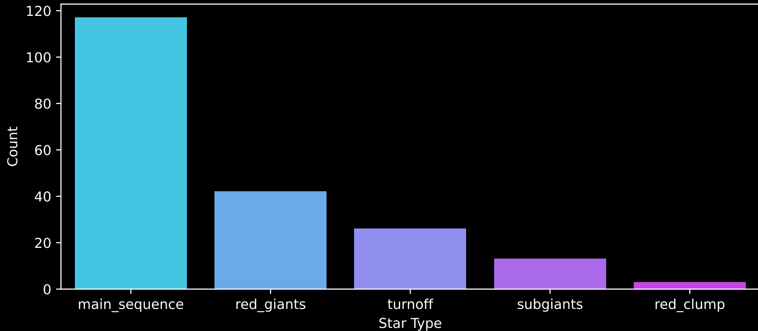
APOGEE DR17 Field: [260+55] Count plot of Star Type
