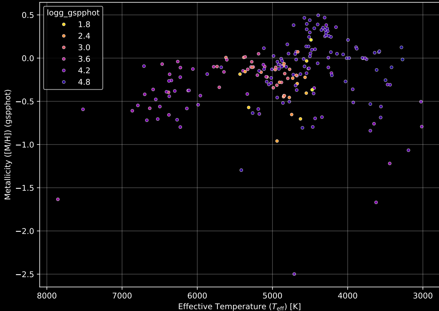
APOGEE DR17 Field: [260+55] Stellar Population Parameters (n= 201)
