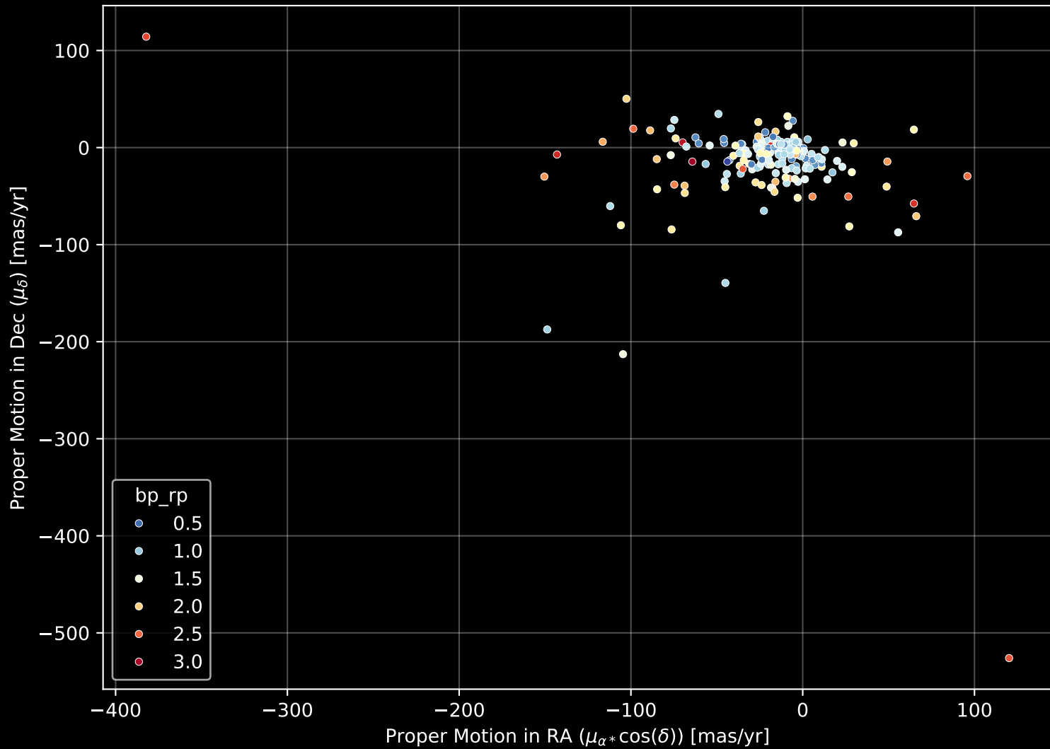
APOGEE DR17 Field: [260+55] Proper Motion Diagram (n= 201)
