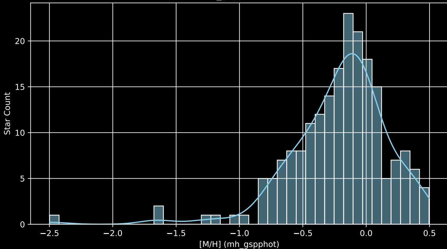
APOGEE DR17 Field: [260+55 [M/H] (mh_gspphot) (n= 201)
