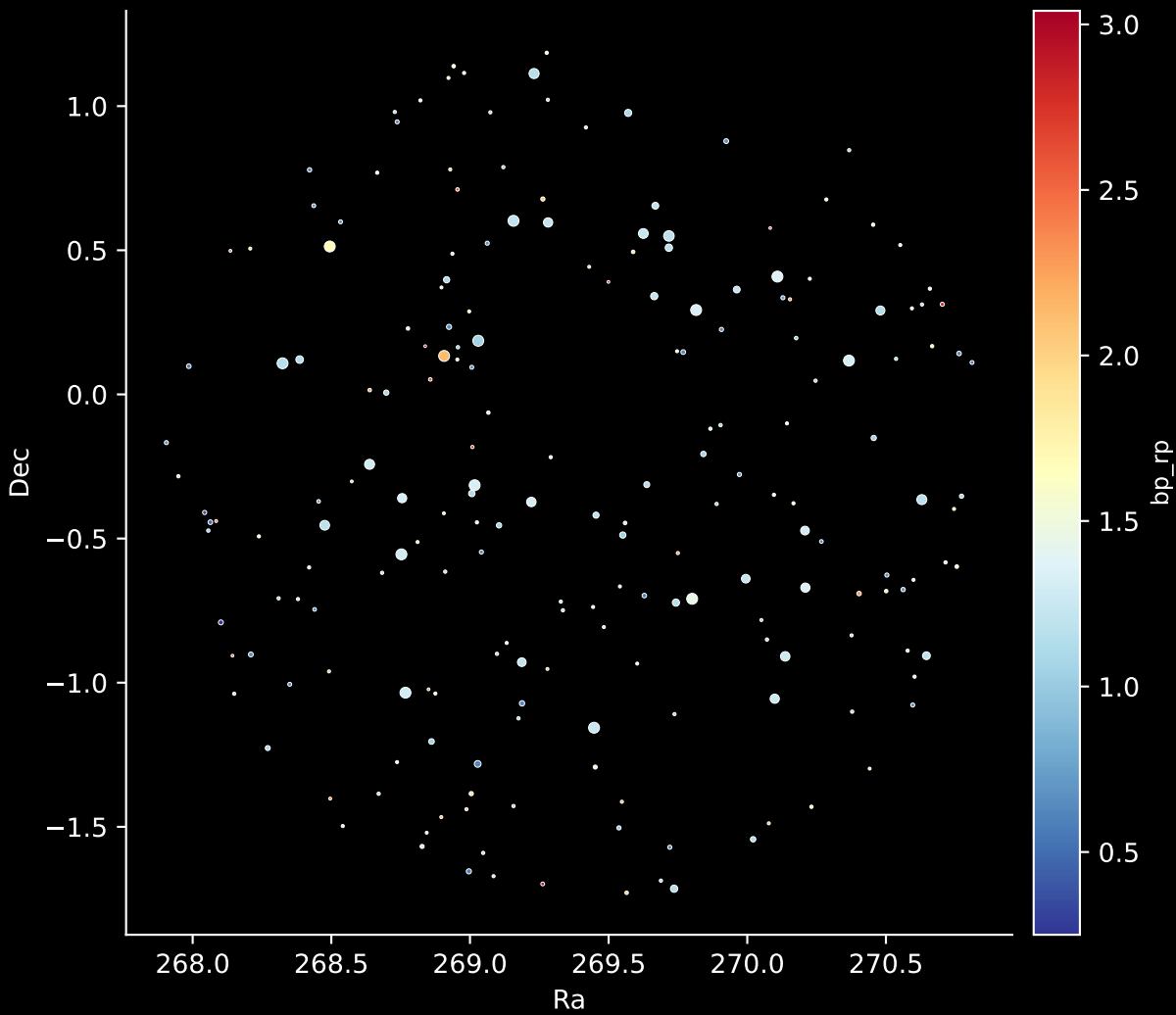
APOGEE DR17 Field: [260+55] Stars: 201
