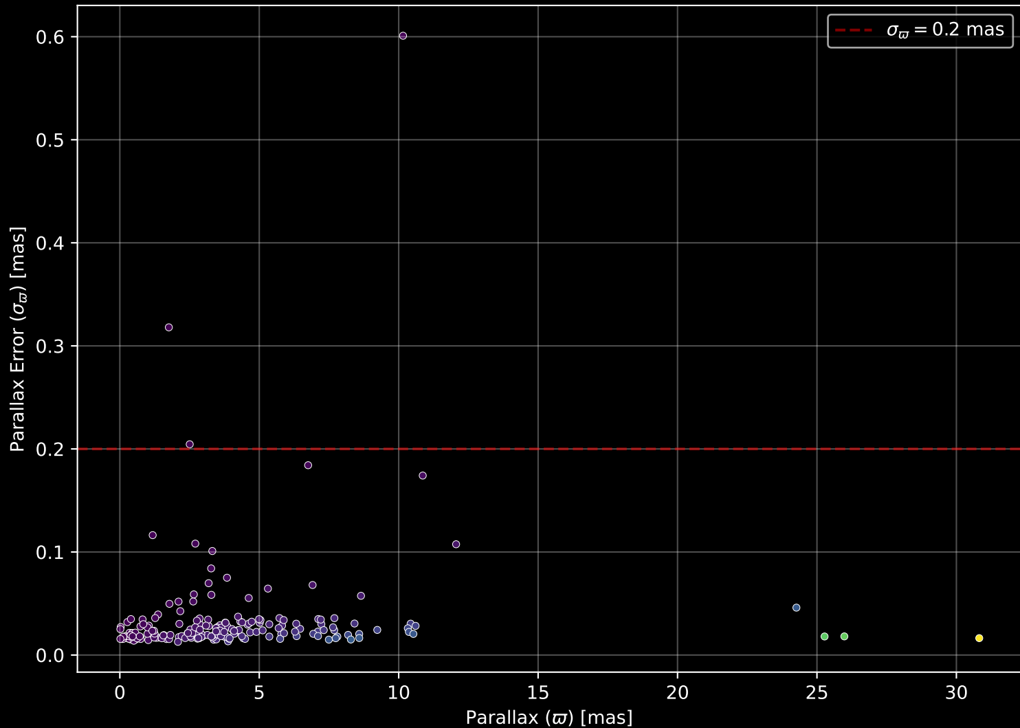
APOGEE DR17 Field: [260+55] Parallax Quality (n= 201)
